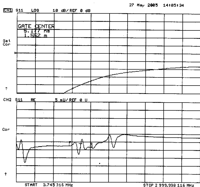
Figure 7 - Adjust Gate to Center DUT
