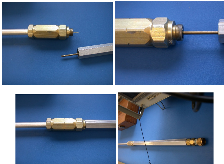
Figure 4 - Connect Precision Airline
