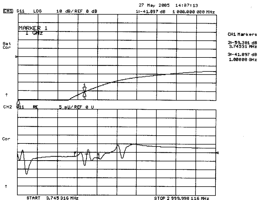
Figure 8 - Worst Case Return Loss
