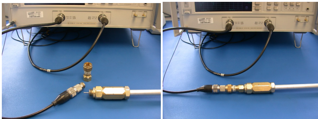
Figure 2 - Interface Calibration
