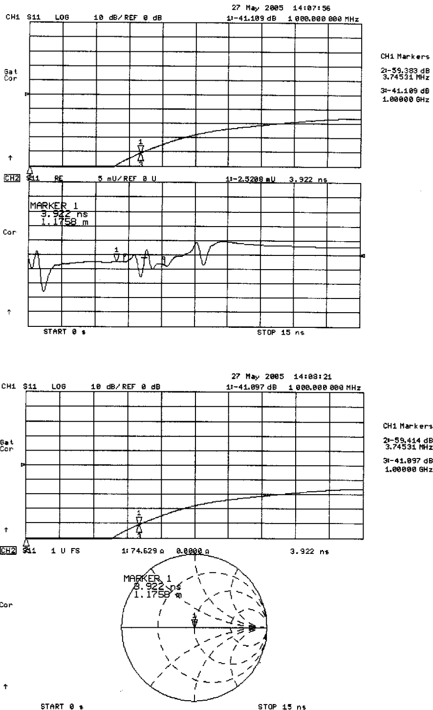
Figure 9 - Cable Impedance
