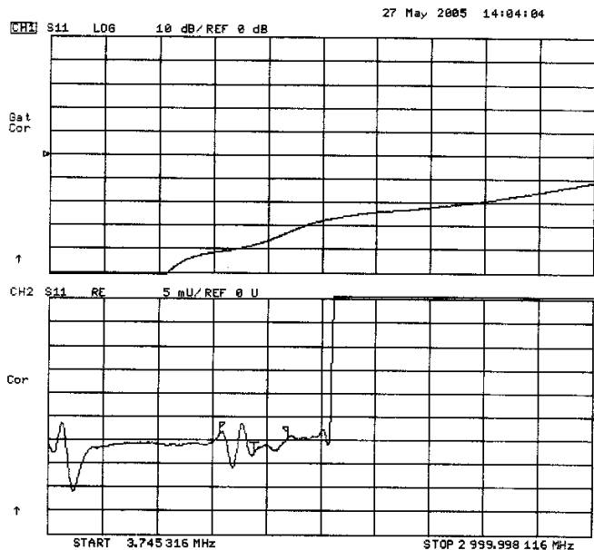
Figure 5 - Open End of Airline Adapter
