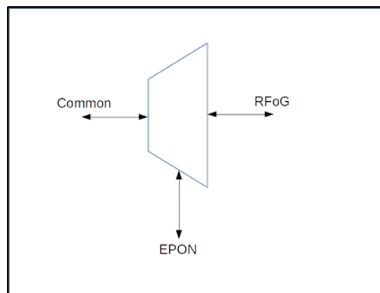
Figure 5 - Optional PON Pass Through Filter Block Diagram
