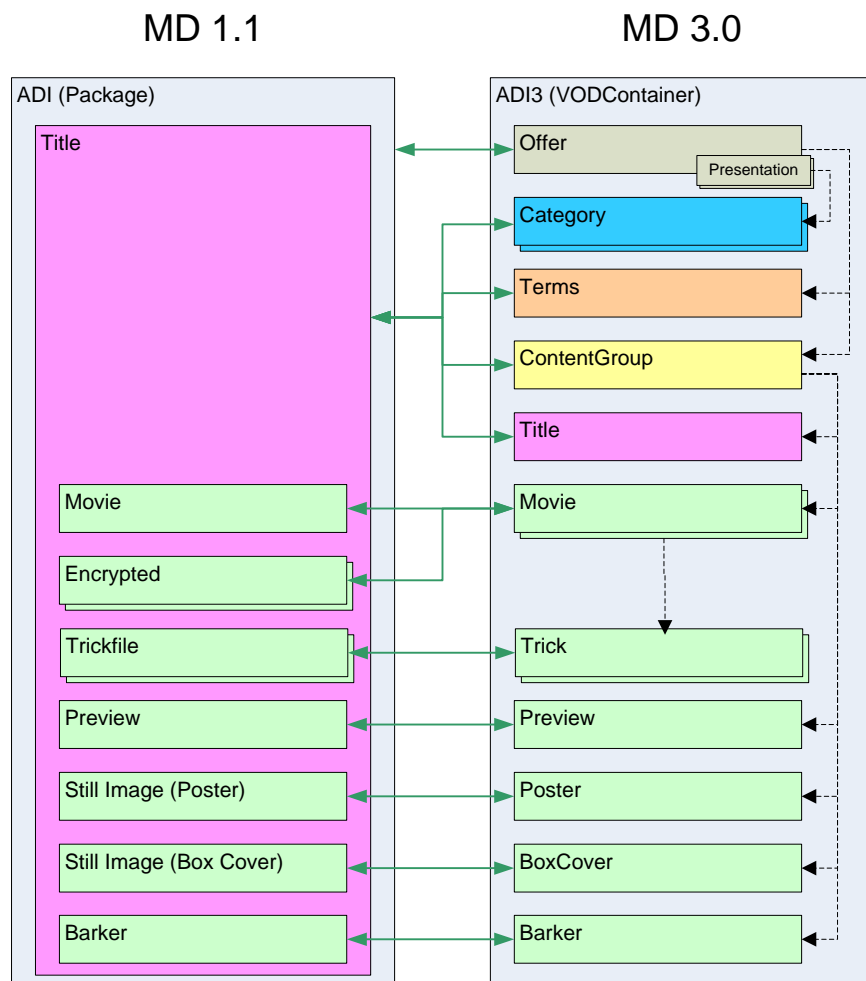
Figure 2 - High level 1.1 ↔ SCTE 236 Mapping
