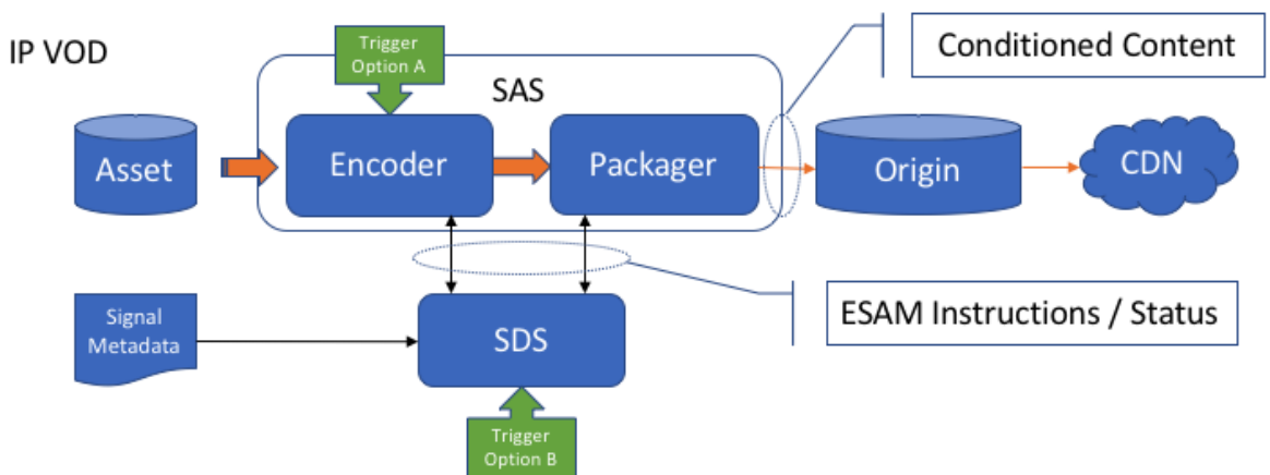
Figure 2 - Example file-based IP Video Application
