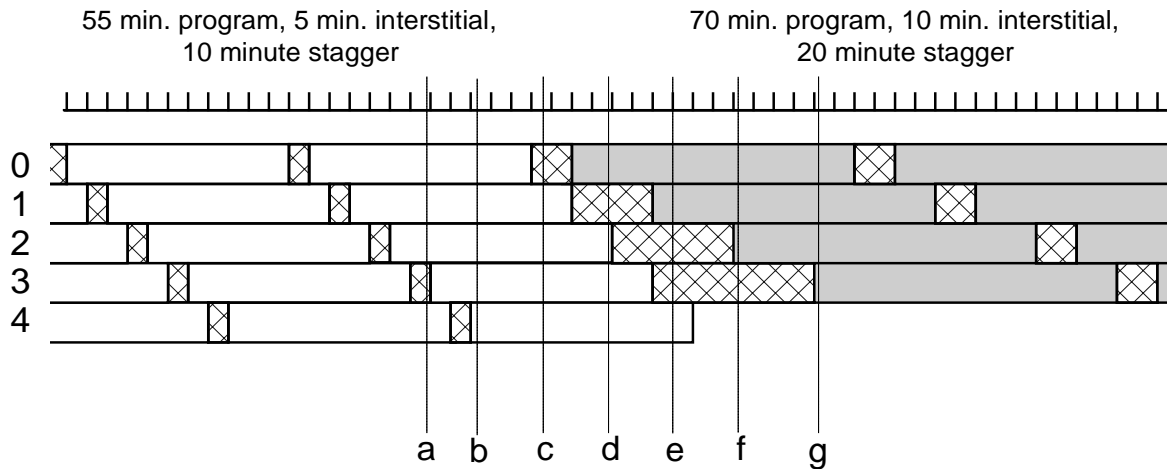
Figure B.3. NVOD Movie Transition Example #2
